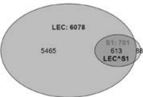
Fig. 7. LEC y Santander-1. NLE = 88 ; PLE = 88 / 701 = 0.126
